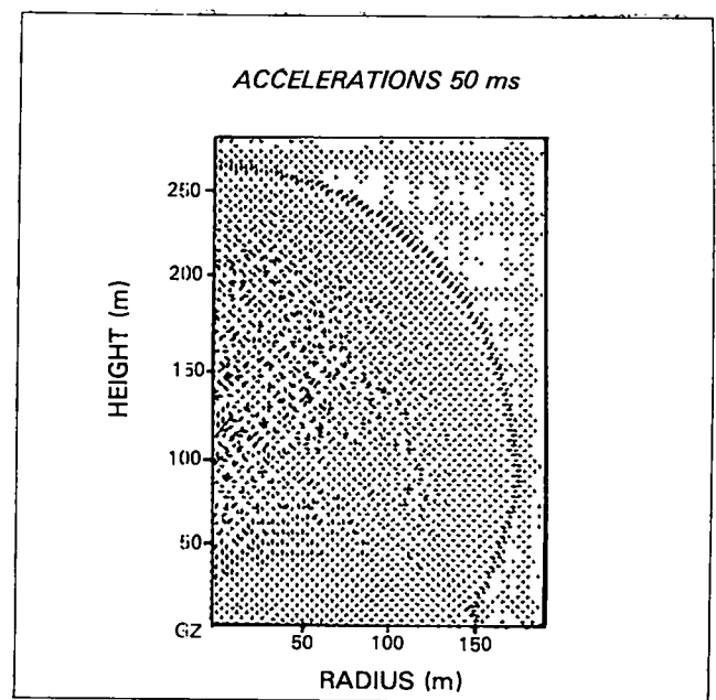
Figure 3. BADGER at 50 ms. The reverse flow is established. Note the counter-clockwise flow in the region within 50 m of GZ. Note in the pressure plot (upper right) that the pressure at GZ has risen, creating a negative gradient. This is an indication of the real transients in the flow.
